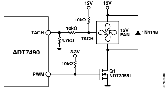
Figure 37. Driving a 3-Wire Fan Using an N-Channel MOSFET
